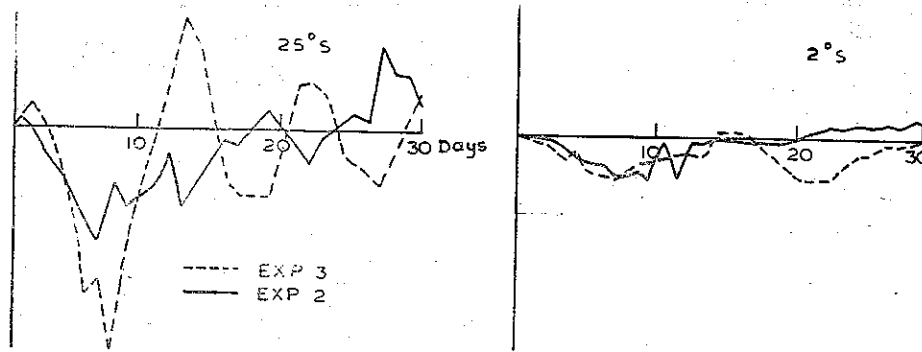
Fig. 8. Comparison of the variation of the momentum flux at 25^{\circ}\text{S} and at the equator for Experiments 2 (solid line) and 3 (dashed line)
