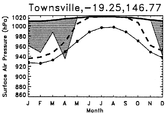
FIG. 3. Seasonal march of MPI predicted by applying the techniques of Holland (1997) and Emanuel (1991) to a number of monthly mean radiosonde soundings in the Australian-southwest Pacific region, together with the observed extreme cyclone intensities (shaded region). The solid line is the ambient surface pressure; the line with dots is the MPI from Emanuel model; the dashed line is the MPI from Holland model [adapted from Tonkin (1996)].
